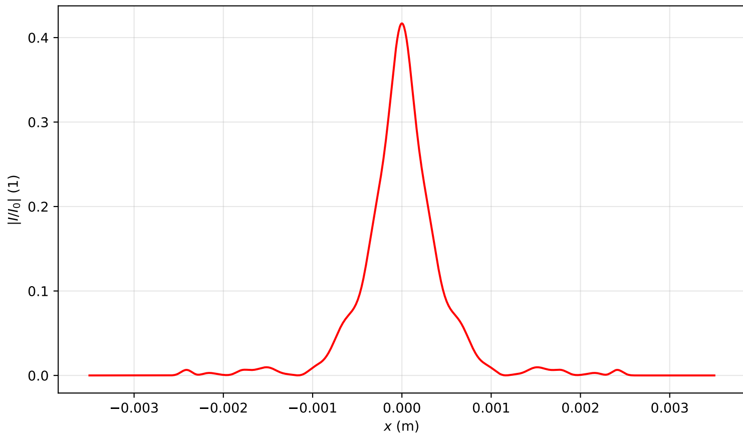
Intensity profile I(x, y = 0, z = 2.229)/I_0 , P_{in}=4.0P_{cr} , artificial time
